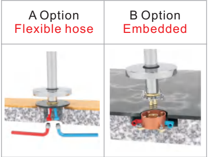
A&B两种安装方式 A&B Two installation models
