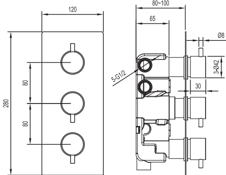
Model: XTZ40704DL5 暗装方形三出水恒温淋浴阀带分流阀-圆手柄 Triple Square Concealed Thermostatic Shower Valve C/W Diverter - Round Handle
