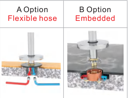
A&B两种安装方式 A&B Two installation models
